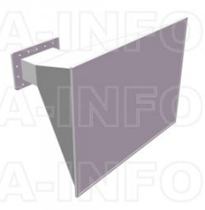
LB-770-15-ASPO Standard Gain Horn Antenna 0.96-1.45GHz 15dB Gain Rectangular Waveguide Interface
